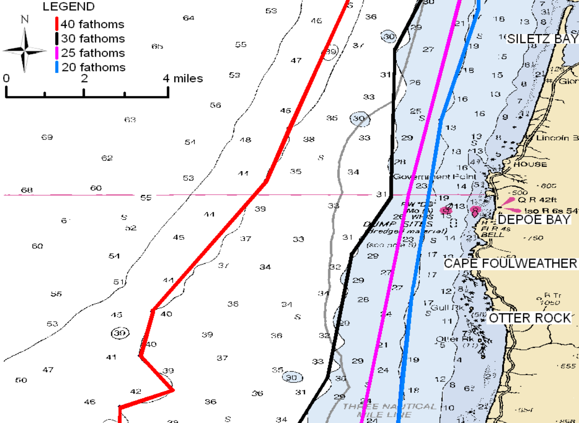
REGULATORY FATHOM CURVES FOR OCEAN SURROUNDING DEPOE BAY
