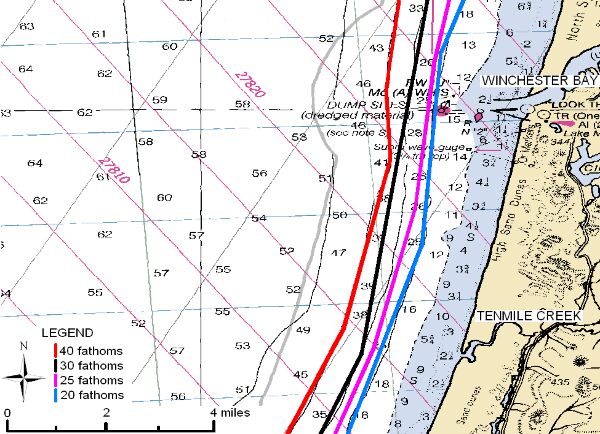
REGULATORY FATHOM CURVES FOR THE OCEAN SURROUNDING WINCHESTER BAY 12
