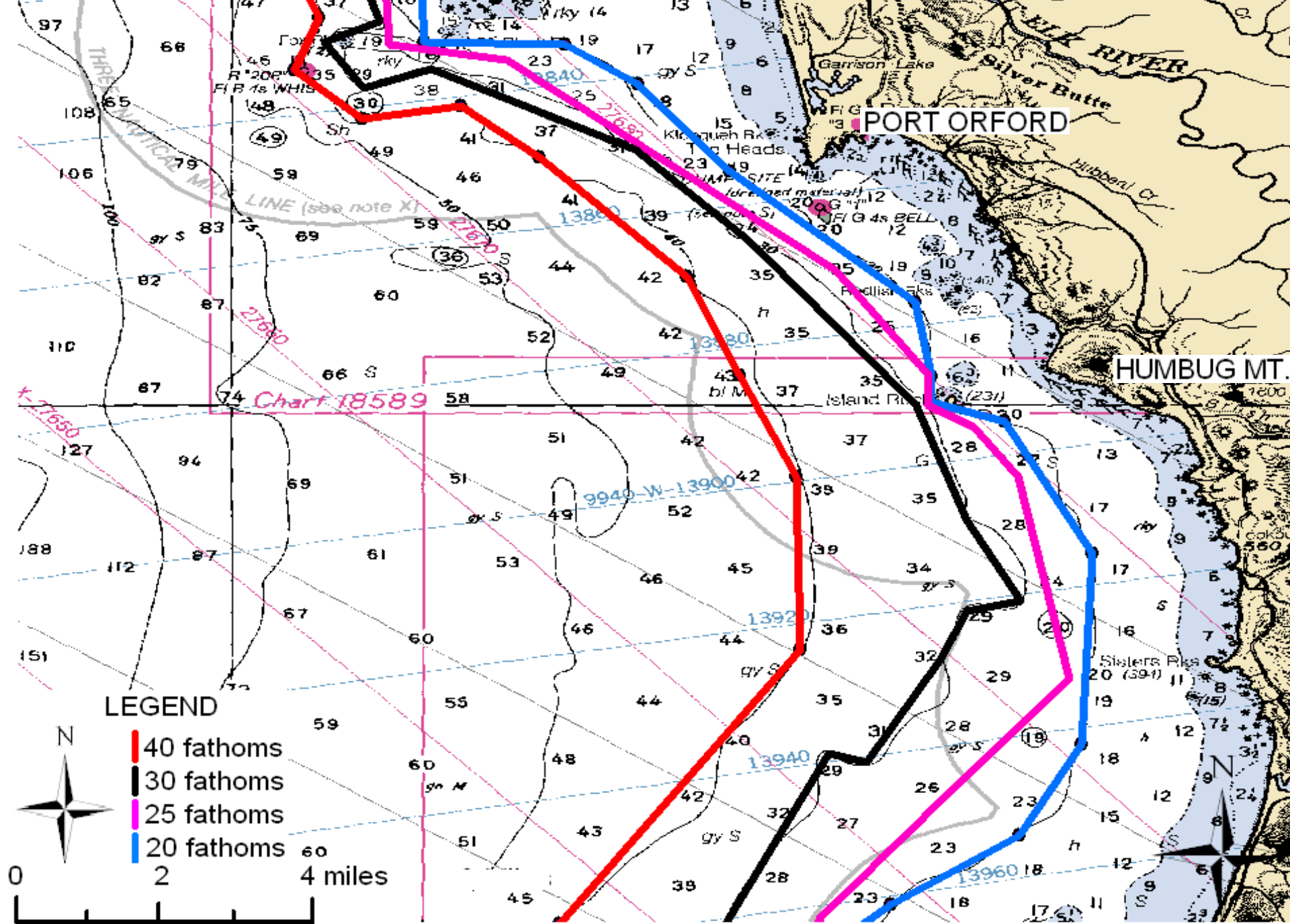
REGULATORY FATHOM CURVES FOR OCEAN SURROUNDING PORT ORFORD
