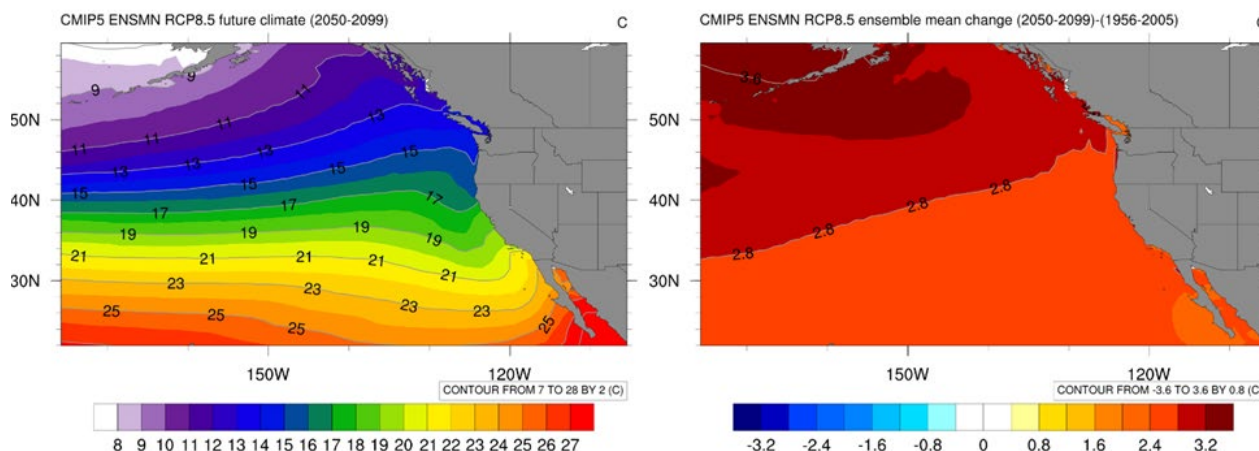
Figure 12. Left Panel: RCP 8.5 future SST for the period 2050-2099; Right Panel: Difference in mean SST between future (2050-2099) and reference period (1956-2005). SST interpolated on a 1°x1° grid for the entire year. Figure downloaded from the Climate Change Web Portal of the NOAA Earth Systems Research Laboratory ( https://www.esrl.noaa.gov/psd/ipcc/ocn/ ).
