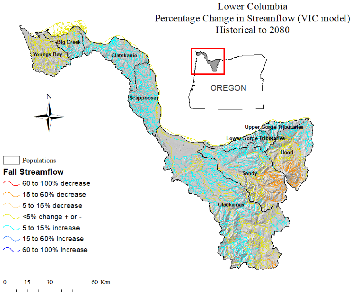
Figure 8. Projected percentage change in median fall stream flow in 2080 relative to the historical baseline (1915–2006) in the Oregon portion of the LCR ESU. Projections were developed using the VIC model (Liang et al. 1994; Hamman et al. 2018) based on the A1B emissions scenario.
