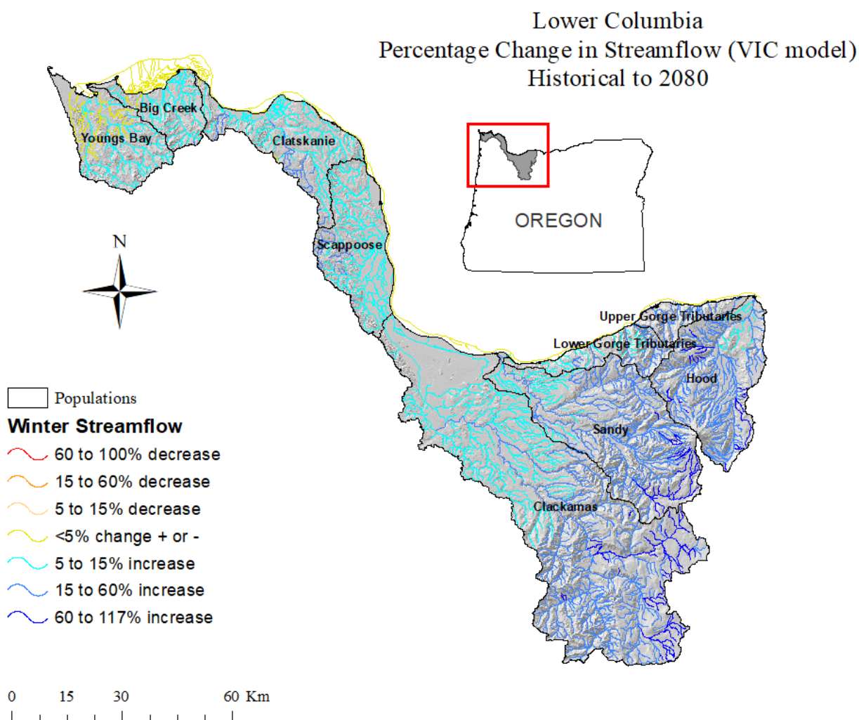
Figure 9. Projected percentage change in median winter stream flow in 2080 relative to the historical baseline (1915–2006) in the Oregon portion of the LCR ESU. Projections were developed using the VIC model (Liang et al. 1994; Hamman et al. 2018) based on the A1B emissions scenario.
