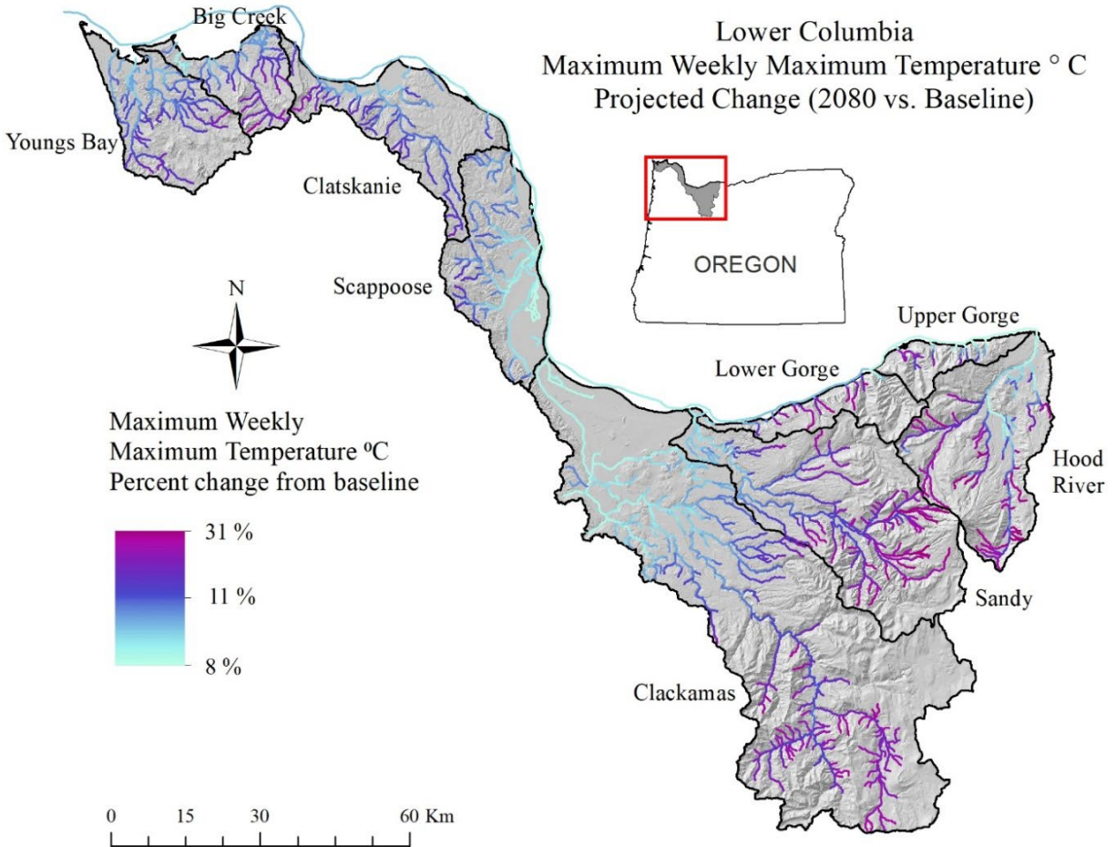
Figure 5. Projected percent change in Maximum Weekly Maximum Temperature (MWMT) estimates (°C) in the 2080s (2070-2099) relative to the baseline (2002-2011 average) under the A1B emissions scenario. Reach specific estimates were obtained from NorWeST (Isaak et al. 2016). NorWeST predictions of stream temperature change in the future assume no changes to surrounding land management, which can either exacerbate or mitigate the changes expected as a result of climate change.
