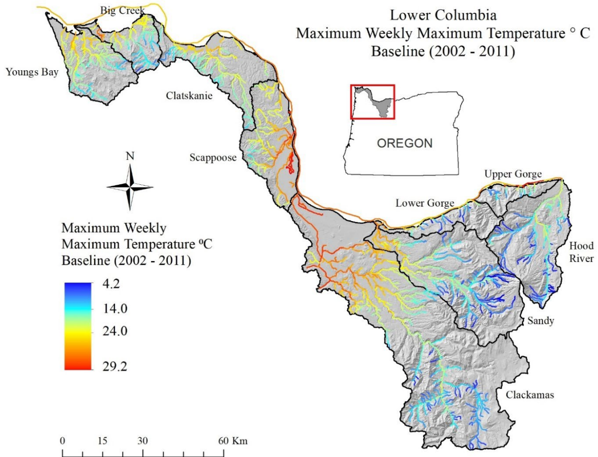
Figure 4. Baseline (2002-2011 average) Maximum Weekly Maximum Temperature (MWMT) estimates (°C) for stream reaches in the Oregon portion of the Lower Columbia River ESU. Reach specific estimates were obtained from NorWeST (Isaak et al. 2016).
