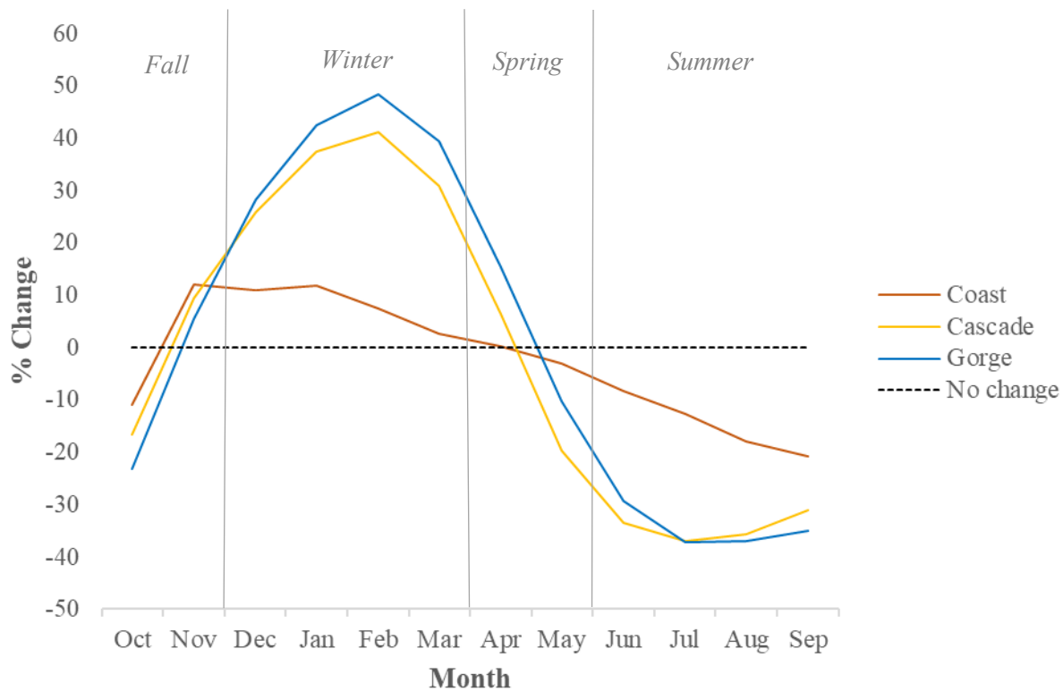
Figure 7. Projected percentage change in median monthly stream flow in 2080 relative to the historical baseline (1915–2006) for the three strata in the Oregon portion of the LCR ESU. Projections were developed using the Variable Infiltration Capacity (VIC) model (Liang et al. 1994; Hamman et al. 2018) based on the A1B emissions scenario.
