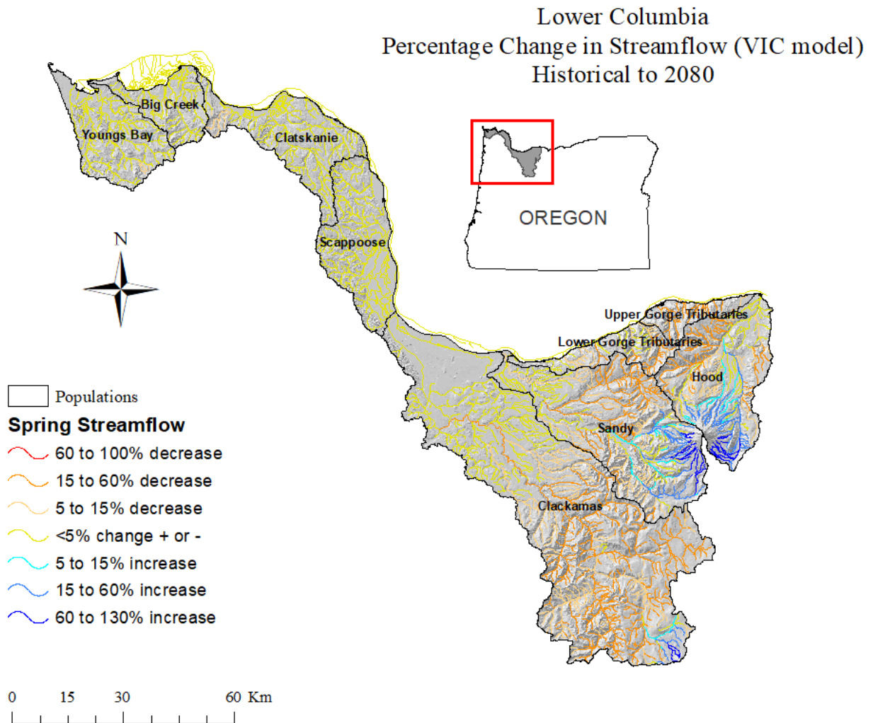
Figure 10. Projected percentage change in median spring stream flow in 2080 relative to the historical baseline (1915–2006) in the Oregon portion of the LCR ESU. Projections were developed using the VIC model (Liang et al. 1994; Hamman et al. 2018) based on the A1B emissions scenario.
