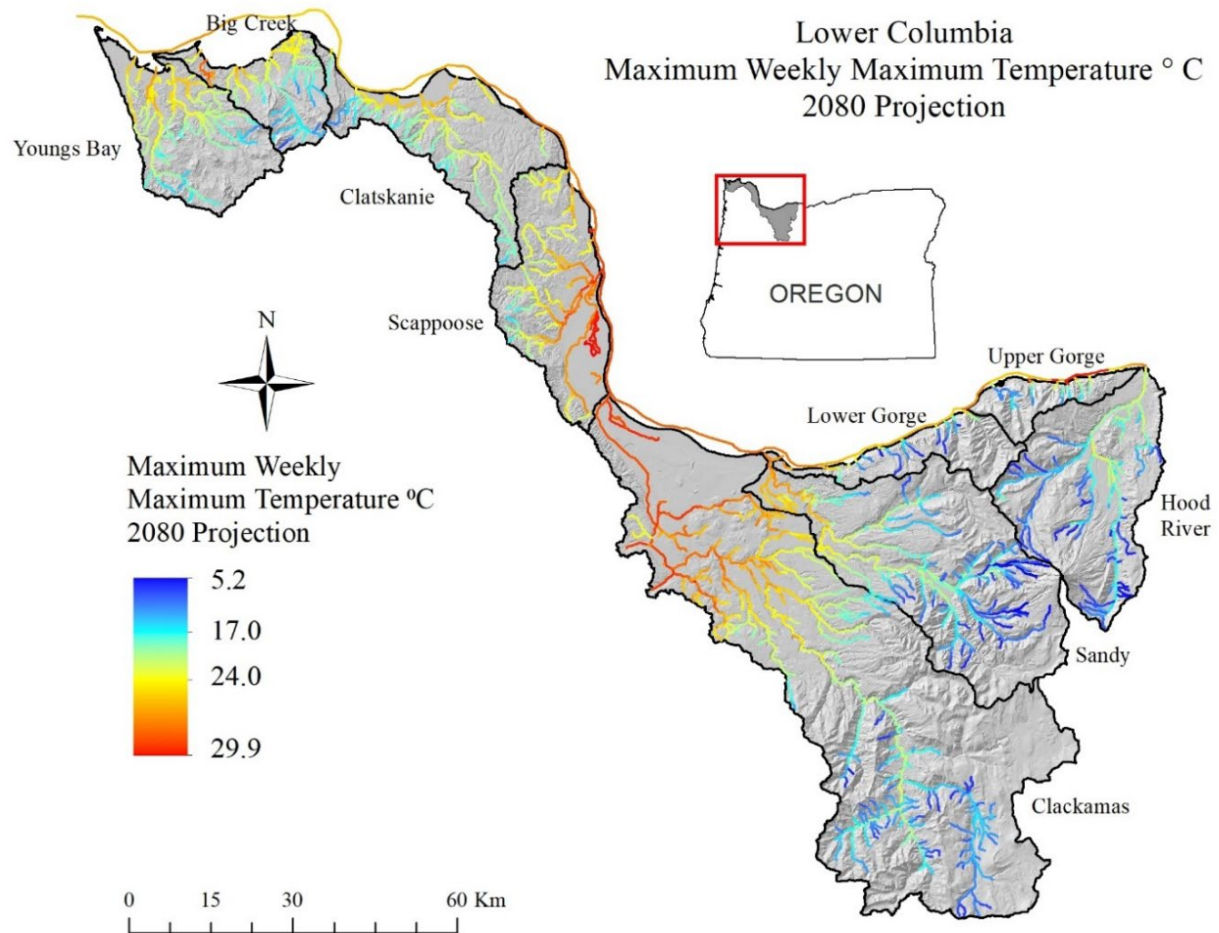
Figure 6. Projected Maximum Weekly Maximum Temperature (MWMT) estimates (°C) in the 2080s (2070-2099) under the A1B emissions scenario. Reach specific estimates were obtained from NorWeST (Isaak et al. 2016). NorWeST predictions of stream temperature change in the future assume no changes to surrounding land management, which can either exacerbate or mitigate the changes expected because of climate change.
