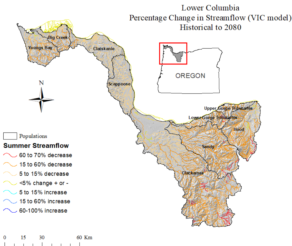
Figure 11. Projected percentage change in median summer stream flow in 2080 relative to the historical baseline (1915–2006) in the Oregon portion of the LCR ESU. Projections were developed using the VIC model (Liang et al. 1994; Hamman et al. 2018) based on the A1B emissions scenario.
