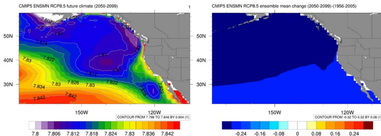
Figure 13. Left Panel: RCP 8.5 future surface pH for the period 2050-2099; Right Panel: Difference in mean surface pH between future (2050-2099) and reference period (1956-2005). Surface pH interpolated on a 1°x1° grid for the entire year. Figure downloaded from: https://www.esrl.noaa.gov/psd/ipcc/ocn/ .
